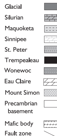
► Figure 2. A. Profile A–A', showing 2.75-dimensional model for southern extent of study area. B. Profile E–E', showing 2.75-dimensional model for northern part of study area. The upper section of each profile shows the aeromagnetic data; the center section, the gravity data. In each section, open circles represent the observed data; the solid line indicates the model-calculated anomaly. The dashed line represents the deviation between the observed and calculated data, and distance from the horizontal gray line indicates greater error. Cumulative error of the model is indicated by the RMSE value. The lower section of each profile illustrates the geologic model; the horizontal distance is relative to the northwest end of the profile, and elevation is above or below mean sea level. Geologic unit categories were modified from the groundwater model layers used by Feinstein and others (2004). nT: nanoTesla.
